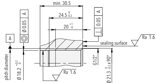
Mounting thread G1/2" 30 mm length (Process connection 94) DIN EN ISO 1179-1
