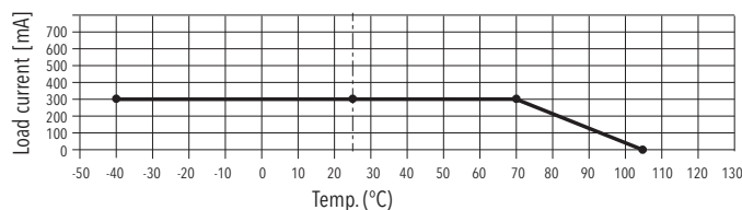
Load depending on ambient temperature
